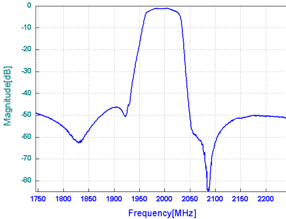
Frequency Response
